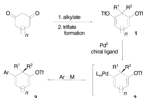
Scheme 1. Desymmetrization-based enantioselective palladium couplings. Tf = trifluoromethanesulfonyl.
