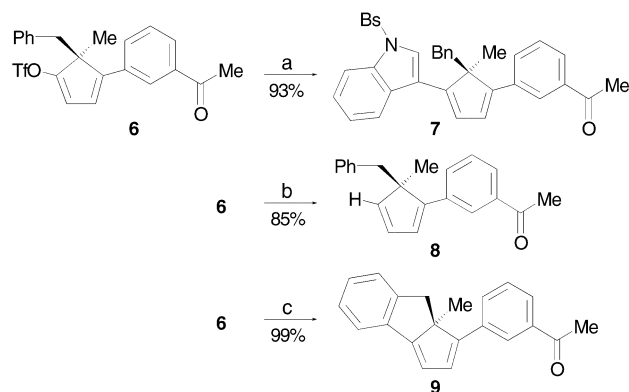
Scheme 3. Functionalization of the monotriflate 6 . Reagents: a) KOH, N -phenylsulfonyl-3-indoleboronic acid, \text{Pd}(\text{OAc})_2 (10 mol%), \text{PPh}_3 (22 mol%), THF, room temperature, 1 h; b) \text{Pd}(\text{OAc})_2 (10 mol%), \text{PPh}_3 (22 mol%), \text{NBu}_3 , \text{HCO}_2\text{H} , DMF, 60°C, 1 h; c) \text{Pd}(\text{OAc})_2 (15 mol%), \text{PPh}_3 (30 mol%), \text{NBu}_3 , DMF, 60°C, 1 h. Bs = benzenesulfonyl. Bn = benzyl.
