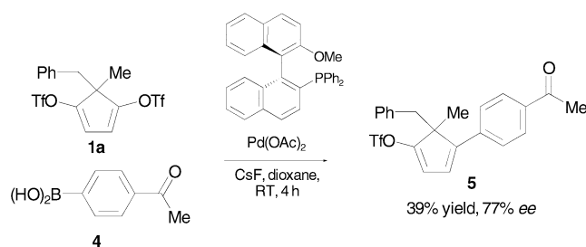
Scheme 2. Desymmetrization of the ditriflate 1a .
